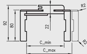
ORB cross-section 075
