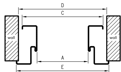
D - width of the assembly hole
