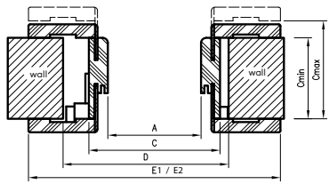
ORB horizontal cross-section
