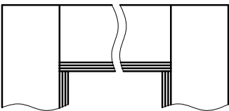
Adjustable door frame connection at an angle of 90° T80 architrave
