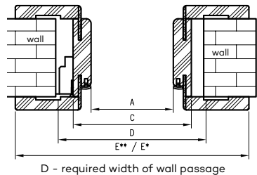
OR/ORC horizontal cross-section
