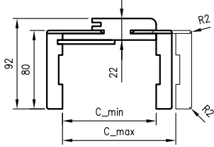
ORB cross-section 075
