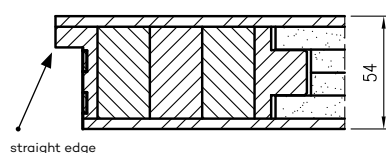
NEFRYT RC3 EI-30 anti-burglary and fire-resistant door leaf
