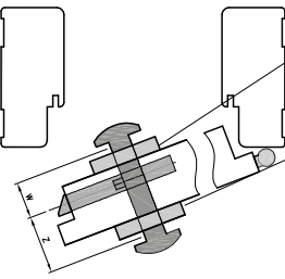
fig. selection of cylinder insert dimension with door knob
