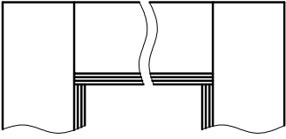
Adjustable non-rebated door frame connection at an angle of 90°** T80 architrave
