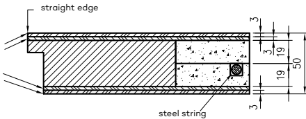
Anti-burglary door leaf Forca B
