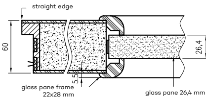
Fire resistant door leaf Olimp EI60
