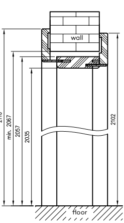
Vertical section of the adjustable tunnel with T63 architrave
