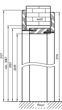
Vertical cross-section of adjustable tunnel with T80 architrave
