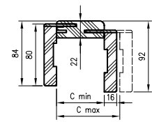
TUN cross-section with T63
