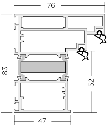
Termo ALU 50mm toktoldó
