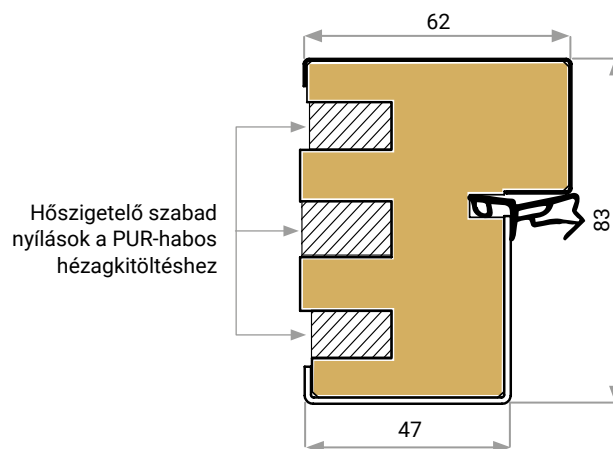
Termo ALU 50mm toktoldó
