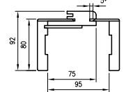
ORB cross-section 075
