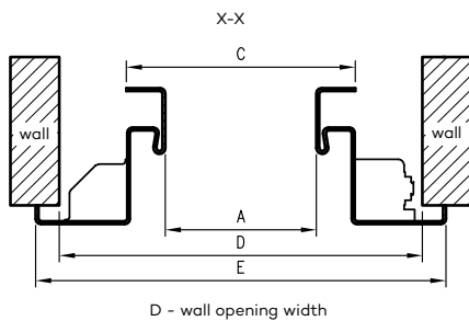
Dimensions for single leaf doors
