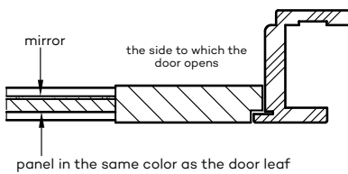
ESTRA 10 door with inverted rebate in the "Reverse" variant
