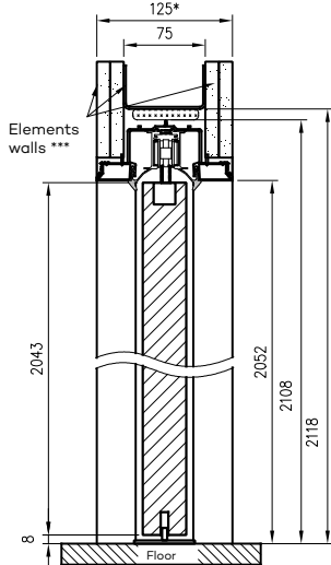
variant of the SL cassette for 125 mm wall
