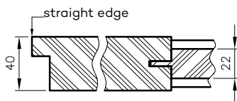
Horizontal cross-section of Nestor
