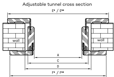
TUN cross-section with T80
