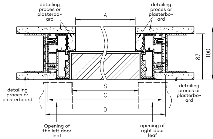
Cross-section of the 50mm non-rebated door - opened outwards
