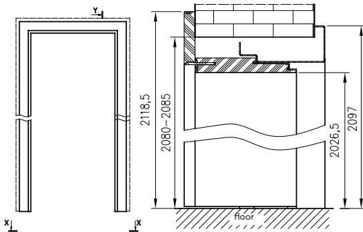
D - width of the assembly hole
