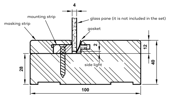
Fig. A cross-section of the transom light/sidelights
