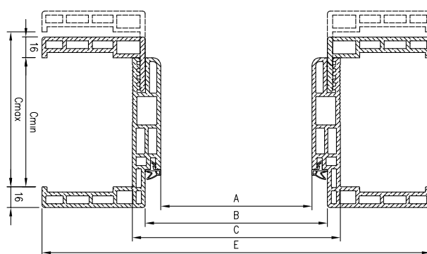
Width of the door frame of a single-leaf rebated door
