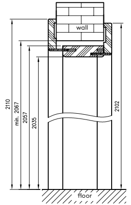
Vertical section of the adjustable tunnel with T63 architrave
