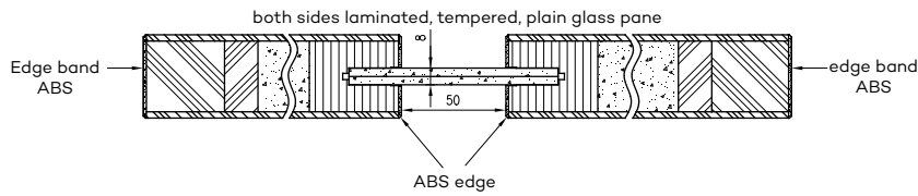
Horizontal cross-section of non-rebated VETRO E doors
