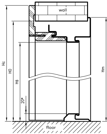
OSH STAND dimensions for double leaf doors
