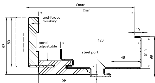
OSHB door frame profile
