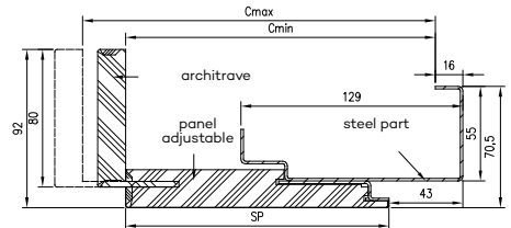
All frames are designed to be mounted on the finished floor.
