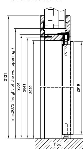
vertical cross-section
