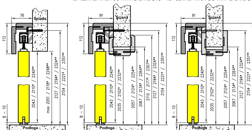
NS - vertical cross-section for tunnel with 63 mm architrave NT - vertical cross-section for tunnel with 80 mm architrave
