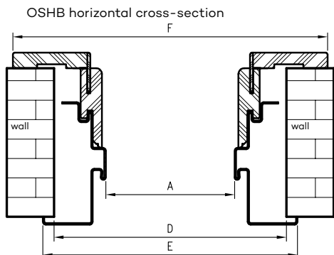
OSHB door frame profile
