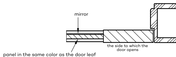
ESTRA 10 doors, non-rebated or rebated, in the "Reverse" variant
