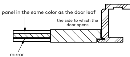
ESTRA 10 door with inverted rebate in the "Reverse" variant
