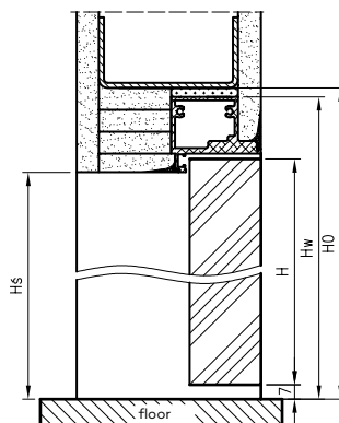
DRE profile for non-rebated outward opening doors
