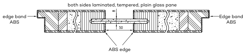
Horizontal cross-section of non-rebated VETRO E doors
